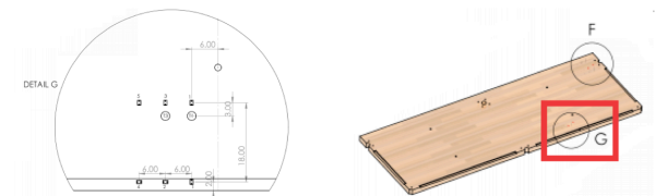
Figure 14. Plywood Spline Probe Locations
