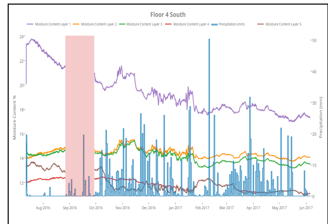
Figure 16. Year Long Moisture Performance
