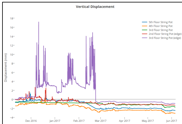
Figure 23. Vertical Displacement Sensor Data
